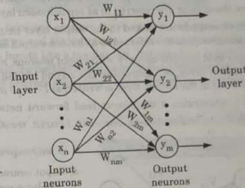
Fig. 1.12.1. Single layer feed forward network.
