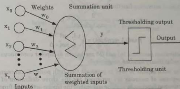
Fig. 1.10.1. Simple model of an artificial neuron.
