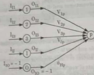
Fig. 2.18.1. Treating threshold in hidden layer.
