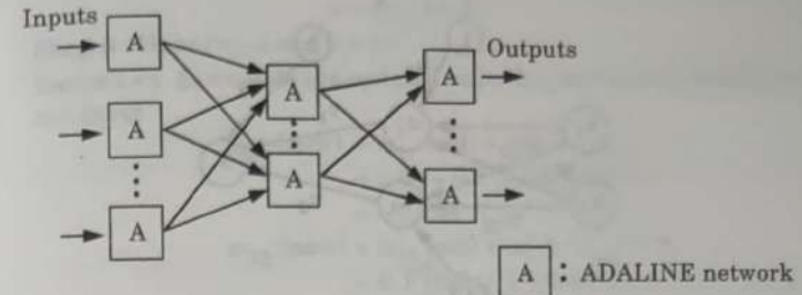
Fig. 2.11.1. MADALINE network.
