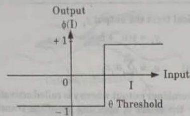
Fig. 1.9.1. Signum function.
