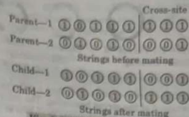
Fig. 5.10.1. Single-site crossover.
