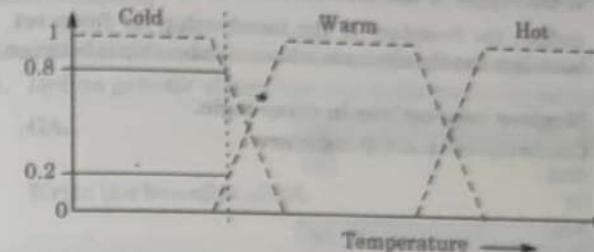
Fig. 1. Membership functions for water temperature.
