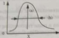
Fig. 4.9.1. Two types of fuzziness.
