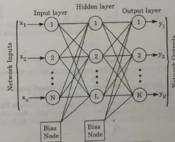
Fig. 1.14.1. Artificial neural network.
