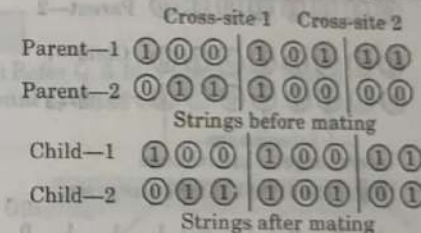
Fig. 5.10.2. Two-point crossover.
