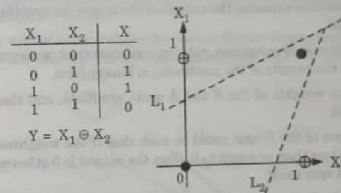
Fig. 2.6.2. Exclusive-OR Function.
