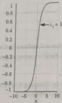
(a) Bipolar sigmoidal function
