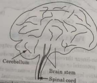
Fig. 1.2.1. Physical structure of the human brain cross-sectional view. Structure of neuron : Refer Q. 1.1, Page 1-2F, Unit-1.
