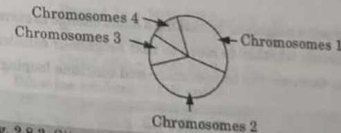
Fig. 2.8.3. Situation after ranking (graph of order numbers).
