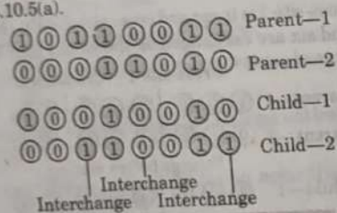
Fig. 5.10.5. (a) Uniform crossover.
