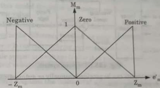
Fig. 4.24.1. Design of membership functions for each situation of e'_m .
