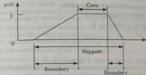
Fig. 4.1.1. Core, support, and boundaries of a fuzzy set.
