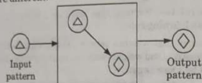
Fig. 1.25.1. Hetero-associative memory.
