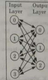
Fig. 1.28.1. BAM network.
