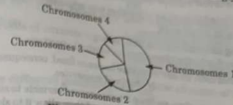
Fig. 2.8.1. Roulette-wheel selection.
