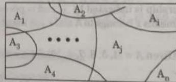
Fig. 3.9.2. Covering of set A.
