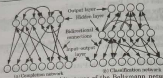
Fig. 3. Two variant architectures of the Boltzmann network.
