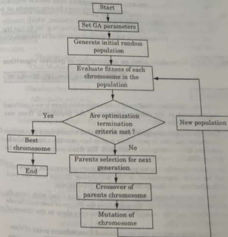
Fig. 5.16.1. Genetic algorithm procedure for TSP.
