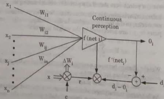
Fig. 1.23.1. Delt learning rule.
