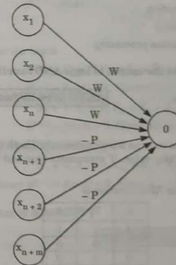
Fig. 2.8.1. Architecture of a McCulloch-Pitts neuron.
