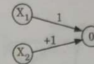
Fig. 2.9.1. McCulloch-Pitts neuron to perform AND function.
