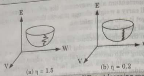
Fig. 2.25.1. Convergence paths for different learning coefficients.
