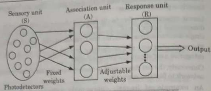
Fig. 2.7.1. Rosenblatt's original perceptron model.
