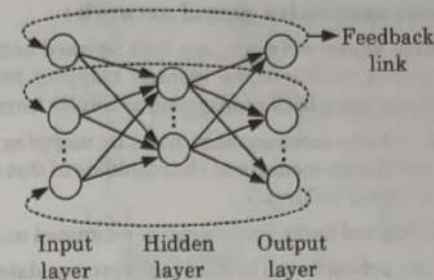
Fig. 1.13.2. A recurrent neural network.
