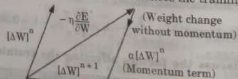
Fig. 2.24.1. Influence of momentum term on weight change.
