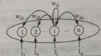
Fig. 1.34.1. Hopfield autoassociative memory architecture.
