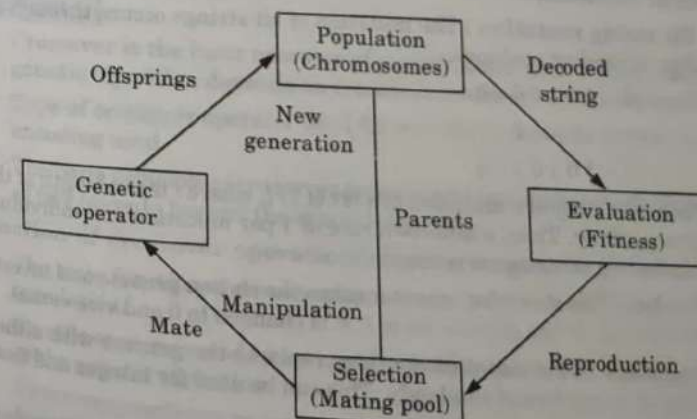
Fig. 5.11.1. The GA cycle.
