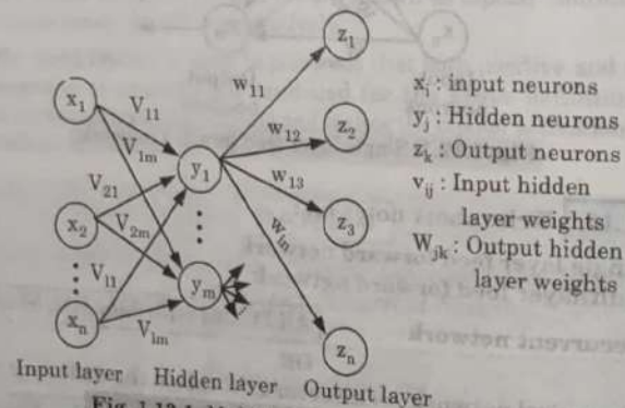
Fig. 1.13.1. Multilayer feed forward network.
