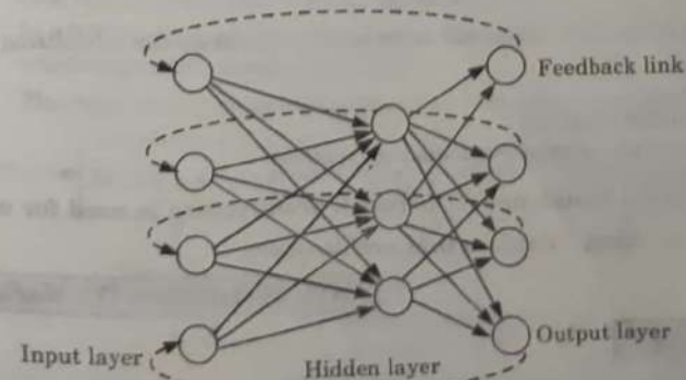
Fig. 1.16.1. A recurrent neural network with self loop.
